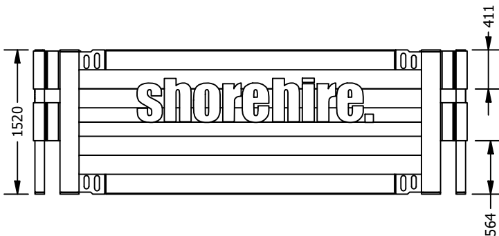
ASSEMBLY-ELEVATION VIEW OPTION-SINGLE STACK
