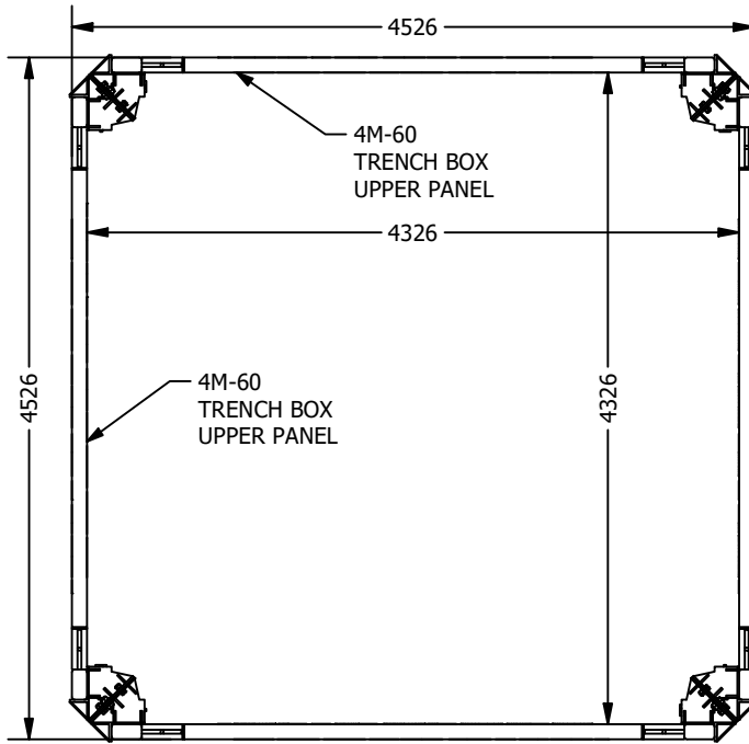
ASSEMBLY-TOP VIEW
