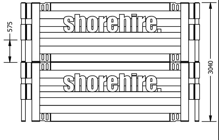
ASSEMBLY-ELEVATION VIEW OPTION-DOUBLE STACK
